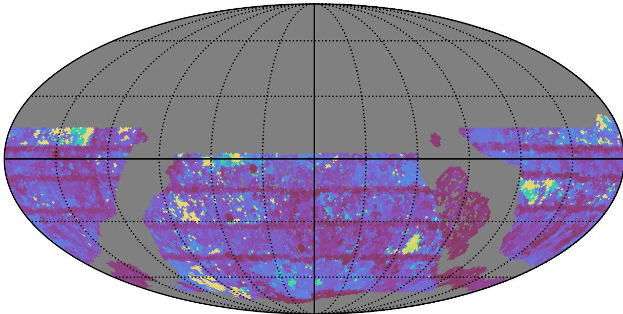
too_elab_r8_d2_giz_v3.4_10yrs WFD i band: Max Inter-Night Gap
