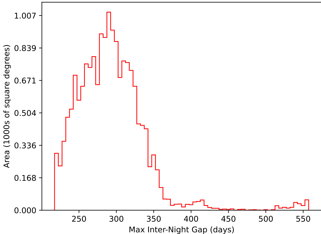
too_elab_r8_d2_giz_v3.4_10yrs WFD i band: Max Inter-Night Gap
