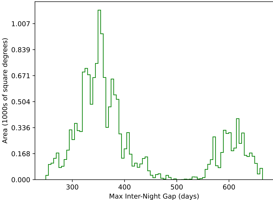
too_elab_r8_d2_giz_v3.4_10yrs WFD g band: Max Inter-Night Gap
