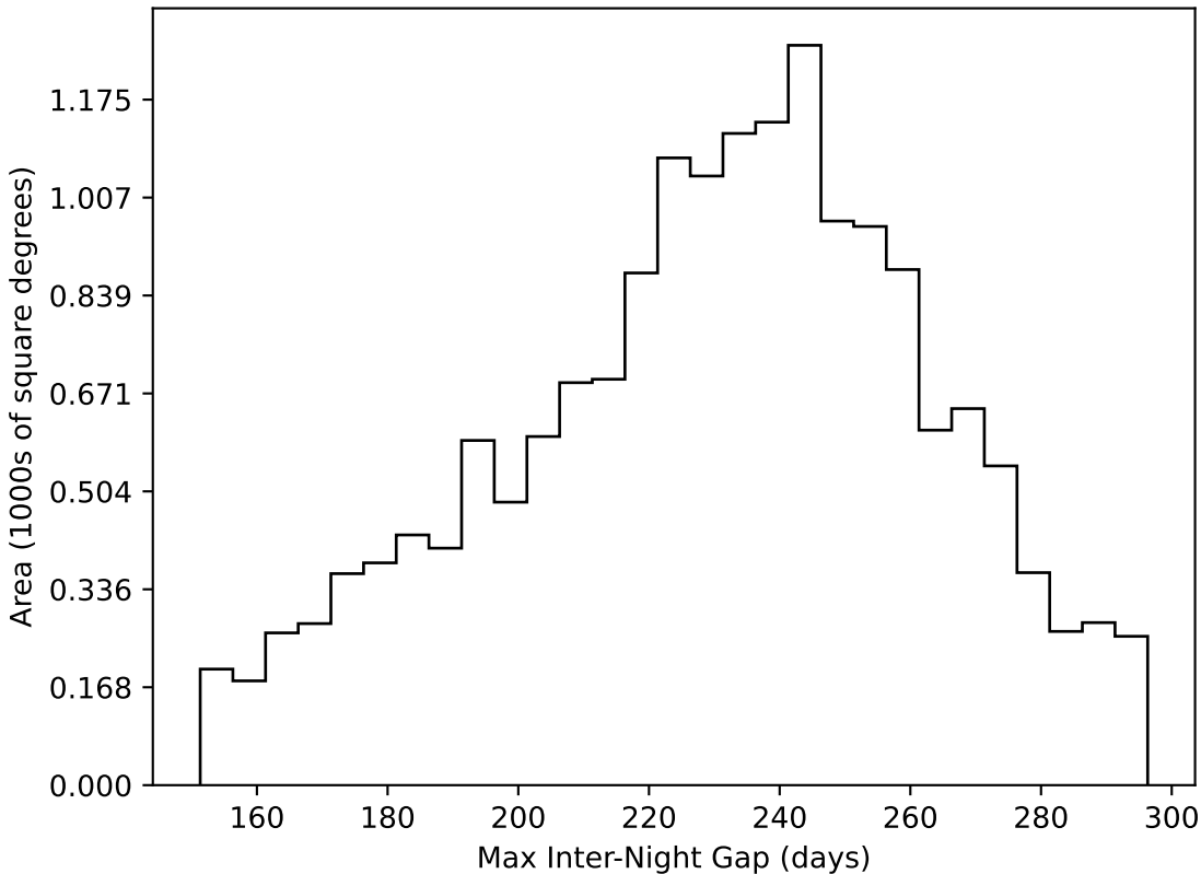
too_elab_r8_d2_giz_v3.4_10yrs WFD all bands: Max Inter-Night Gap
