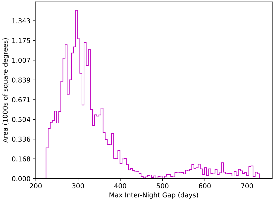
too_elab_r8_d2_giz_v3.4_10yrs All sky z band: Max Inter-Night Gap
