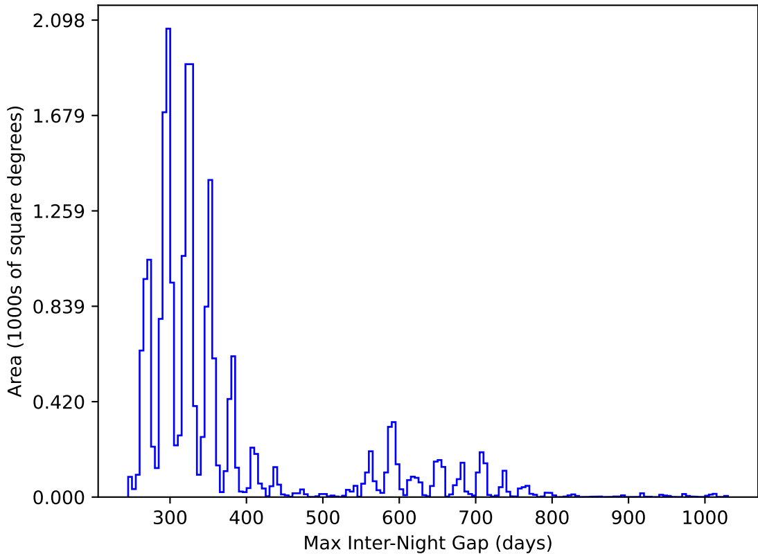
too_elab_r8_d2_giz_v3.4_10yrs All sky y band: Max Inter-Night Gap
