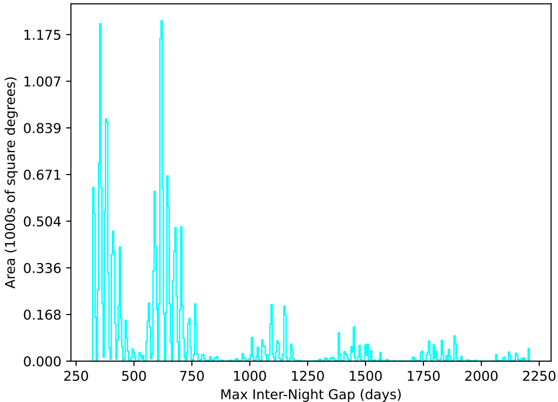
too_elab_r8_d2_giz_v3.4_10yrs All sky u band: Max Inter-Night Gap
