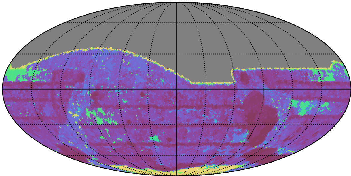
too_elab_r8_d2_giz_v3.4_10yrs All sky r band: Max Inter-Night Gap
