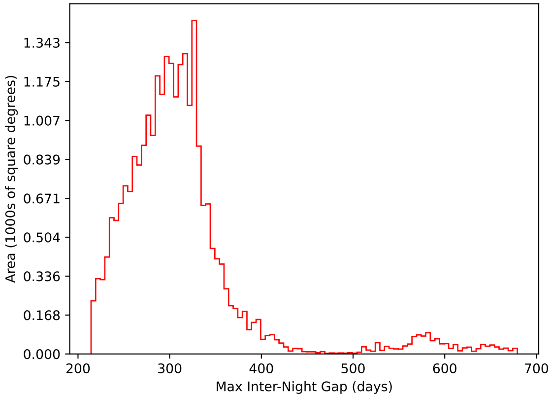
too_elab_r8_d2_giz_v3.4_10yrs All sky i band: Max Inter-Night Gap
