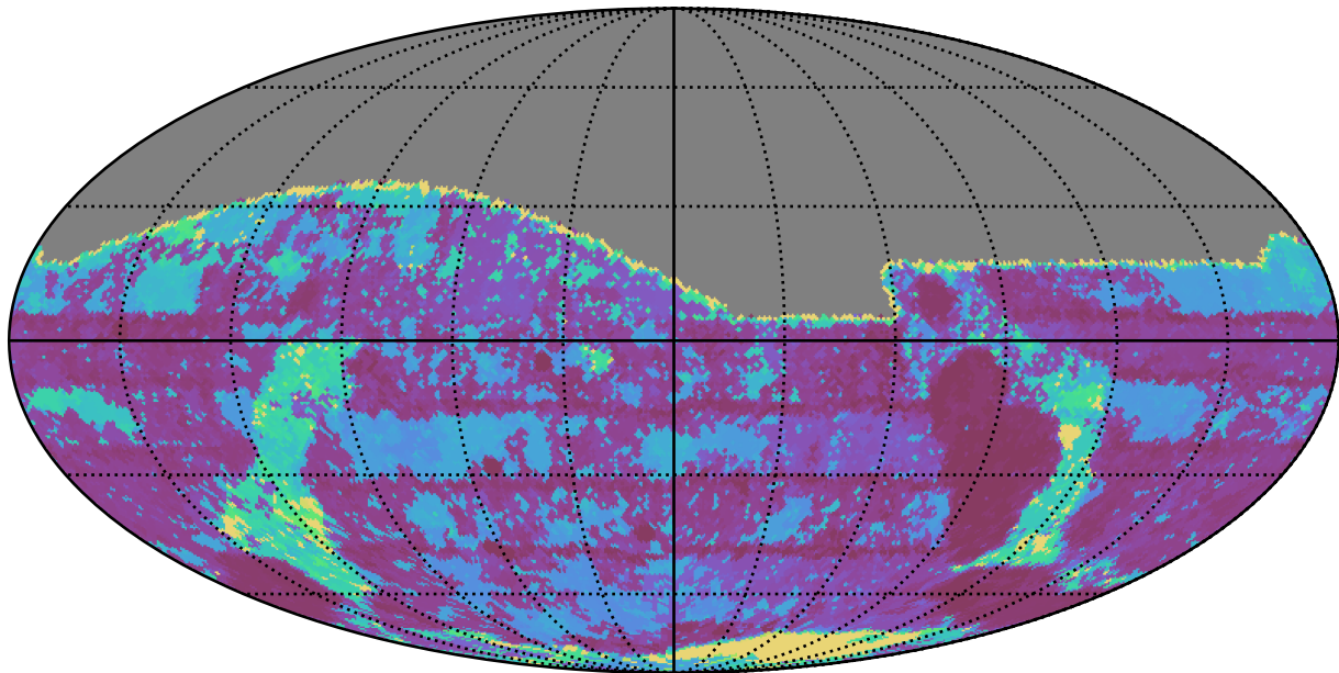
too_elab_r8_d2_giz_v3.4_10yrs All sky g band: Max Inter-Night Gap
