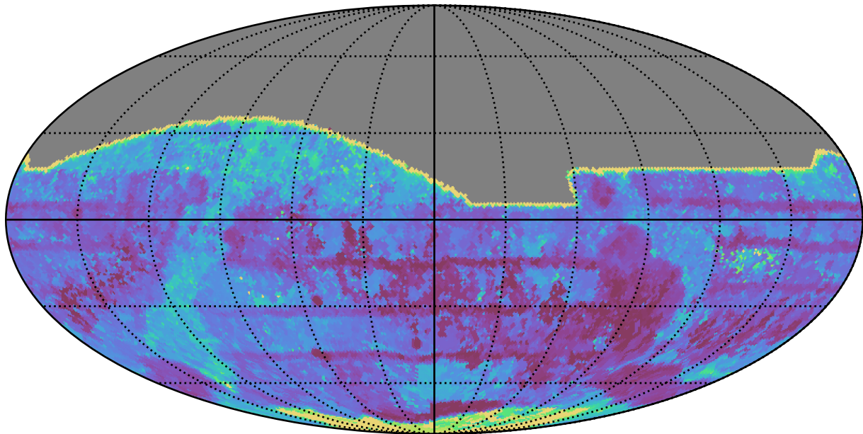
too_elab_r8_d2_giz_v3.4_10yrs All sky all bands: Max Inter-Night Gap
