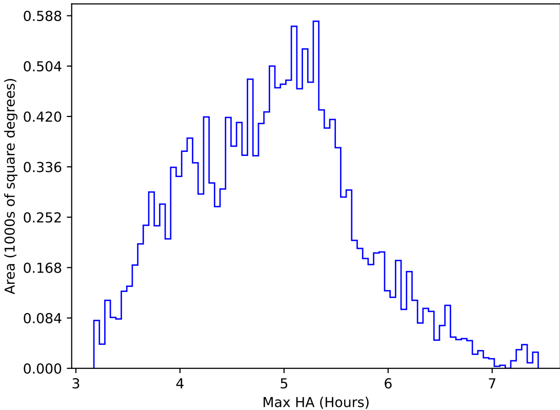
too_elab_r8_d2_giz_v3.4_10yrs WFD z band: Max HA
