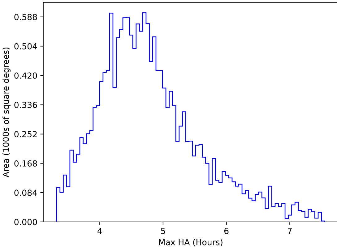
too_elab_r8_d2_giz_v3.4_10yrs WFD y band: Max HA
