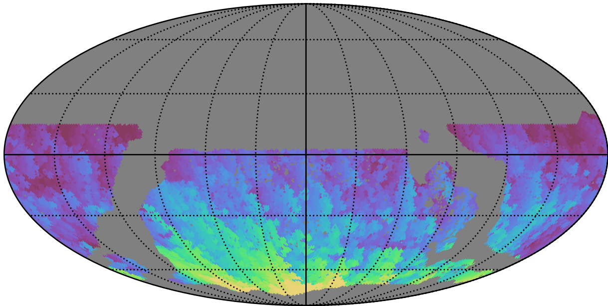
too_elab_r8_d2_giz_v3.4_10yrs WFD r band: Max HA
