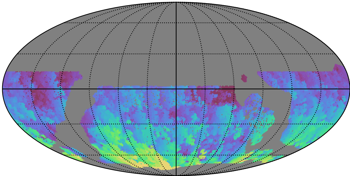
too_elab_r8_d2_giz_v3.4_10yrs WFD g band: Max HA
