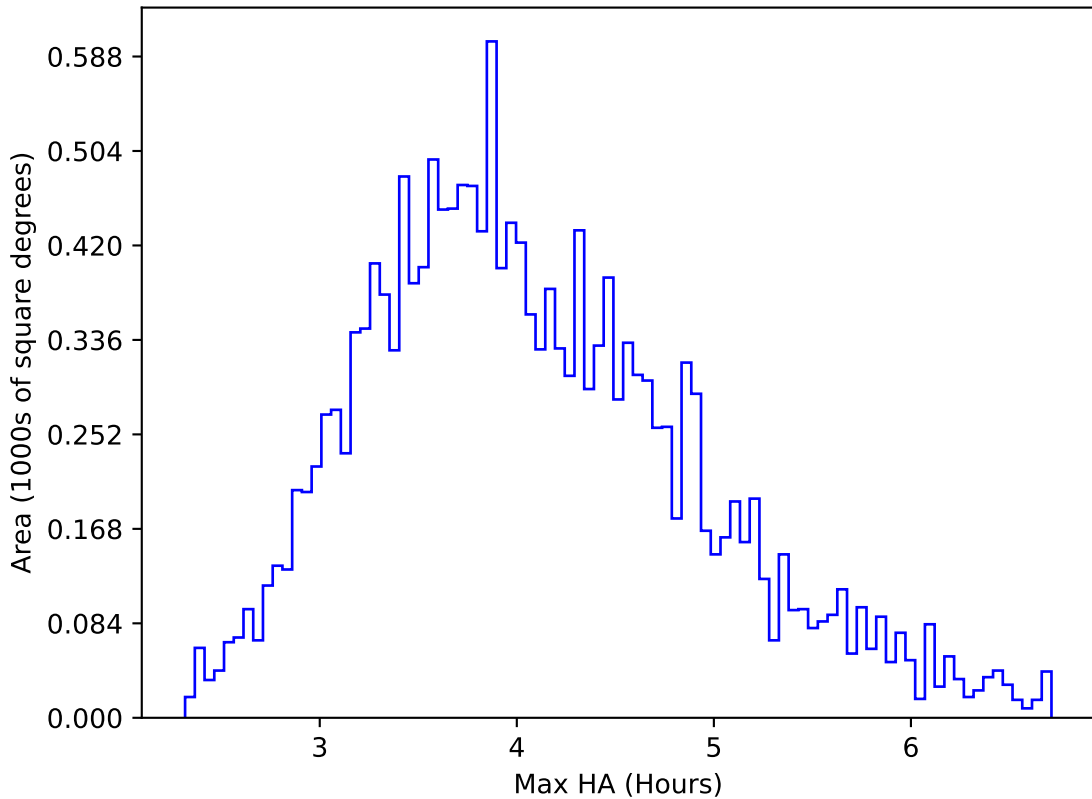
too_elab_r8_d2_giz_v3.4_10yrs WFD g band: Max HA
