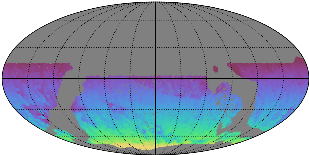
too_elab_r8_d2_giz_v3.4_10yrs WFD all bands: Max HA
