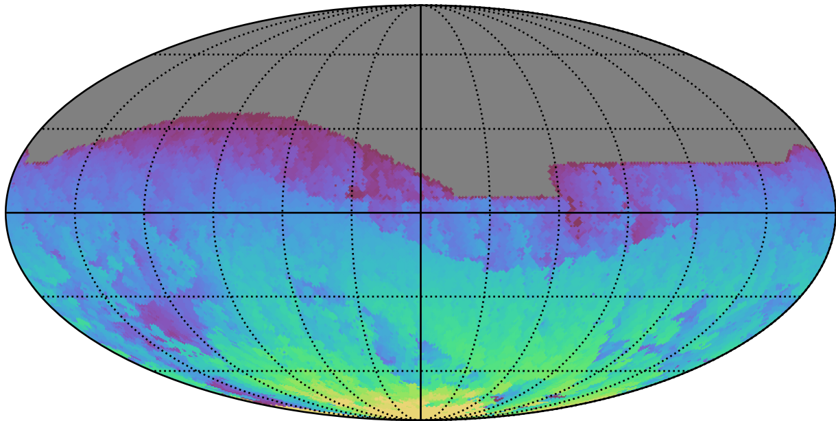
too_elab_r8_d2_giz_v3.4_10yrs All sky z band: Max HA
