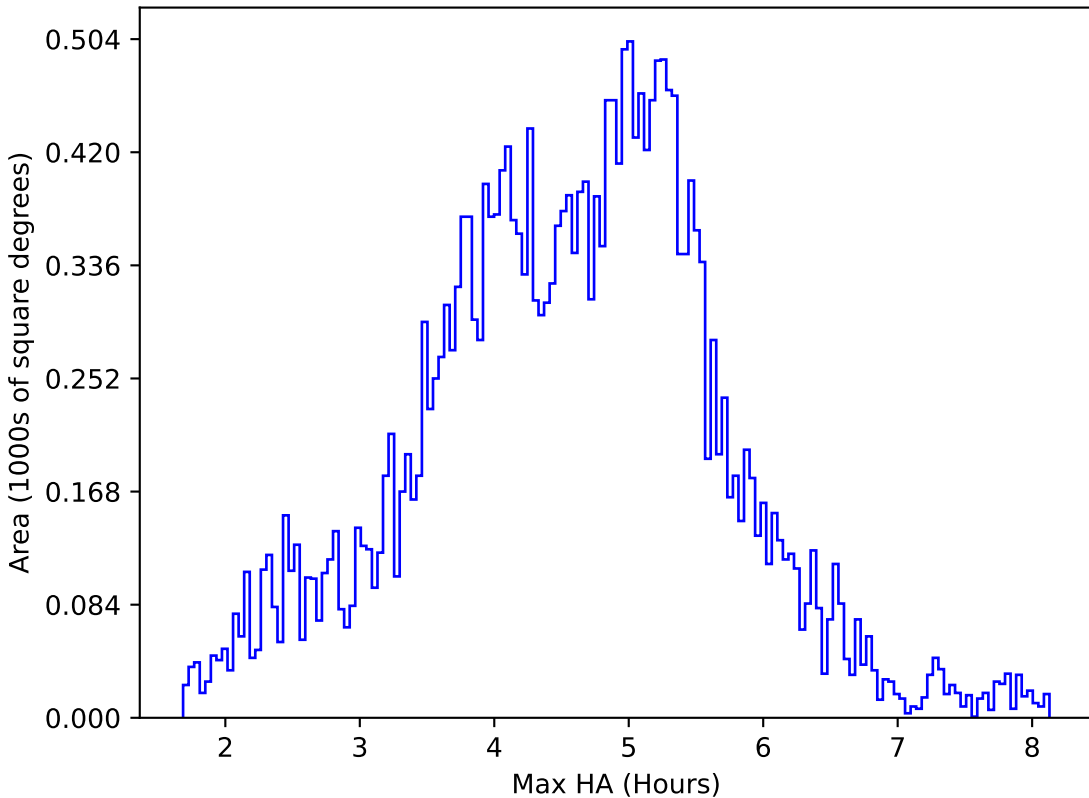
too_elab_r8_d2_giz_v3.4_10yrs All sky z band: Max HA
