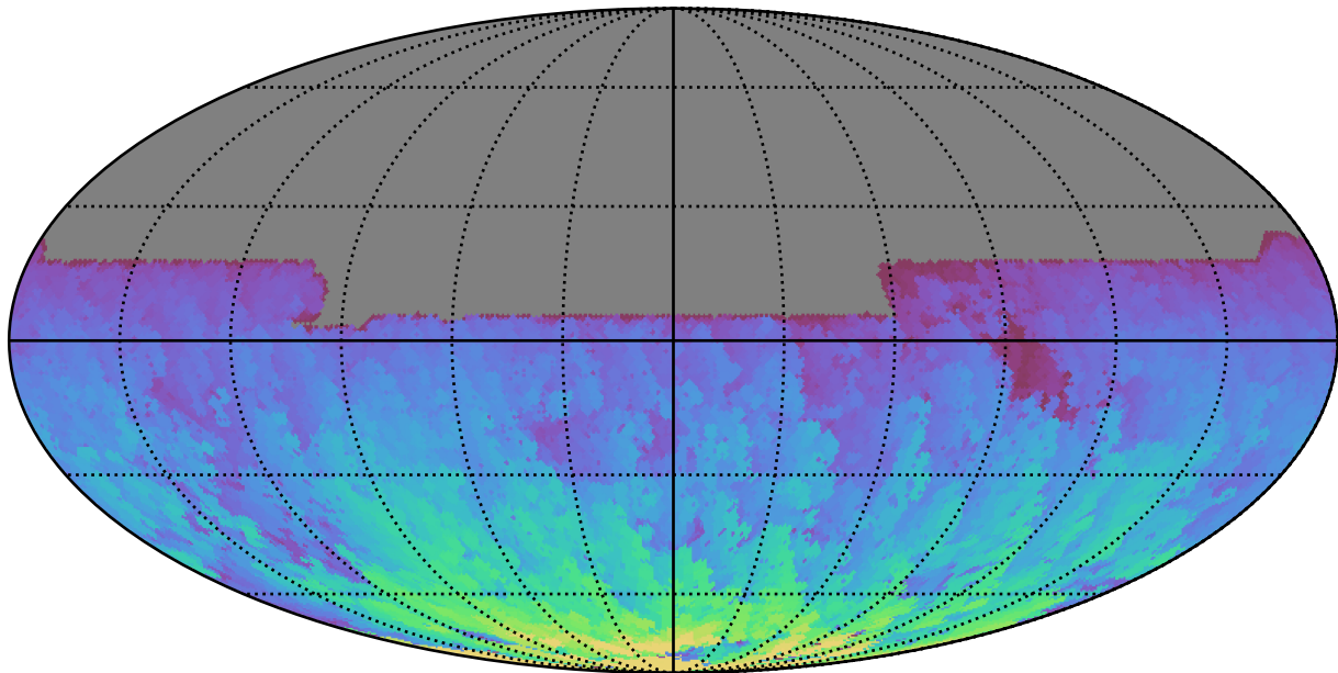
too_elab_r8_d2_giz_v3.4_10yrs All sky y band: Max HA
