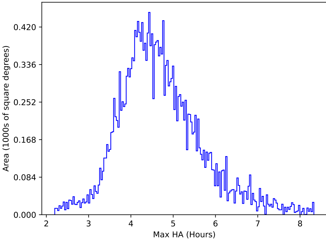
too_elab_r8_d2_giz_v3.4_10yrs All sky y band: Max HA
