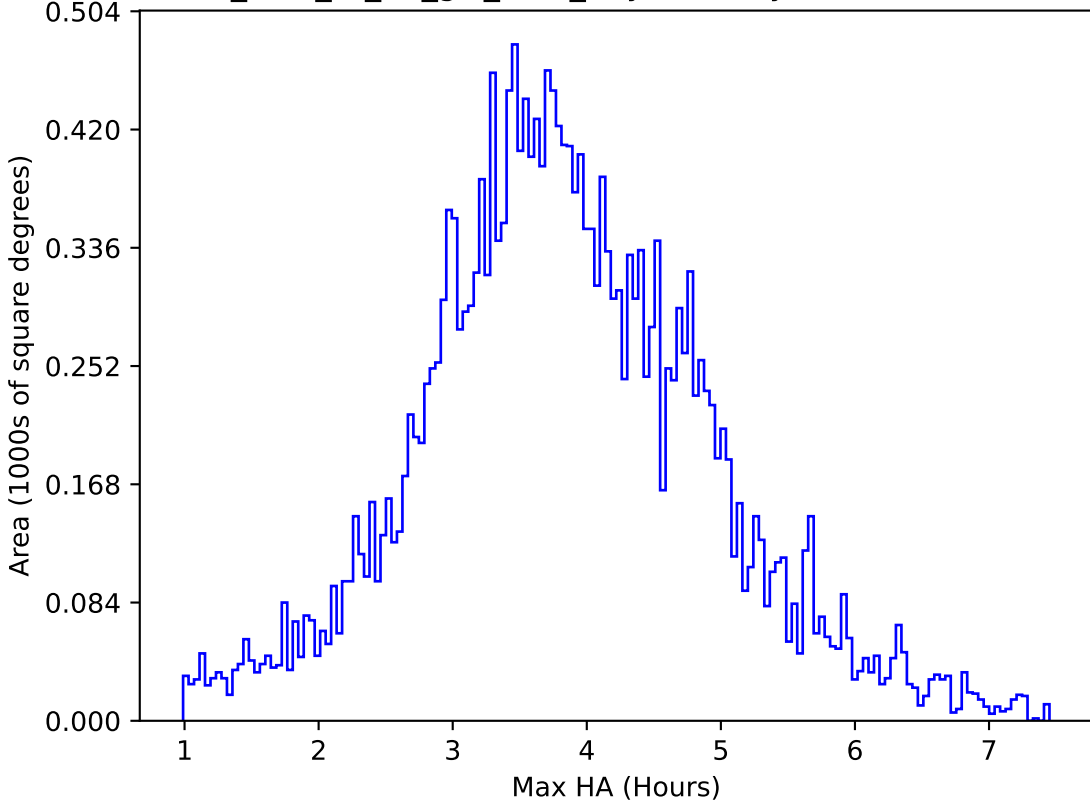
too_elab_r8_d2_giz_v3.4_10yrs All sky u band: Max HA
