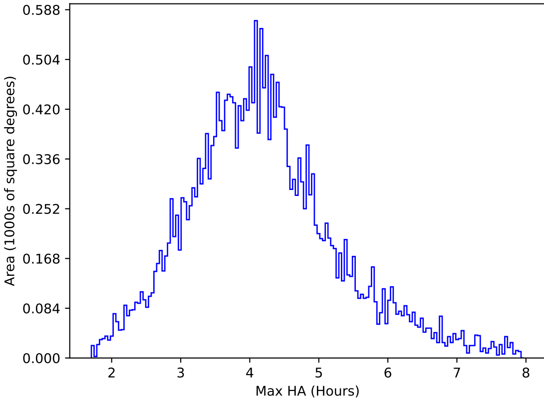
too_elab_r8_d2_giz_v3.4_10yrs All sky r band: Max HA
