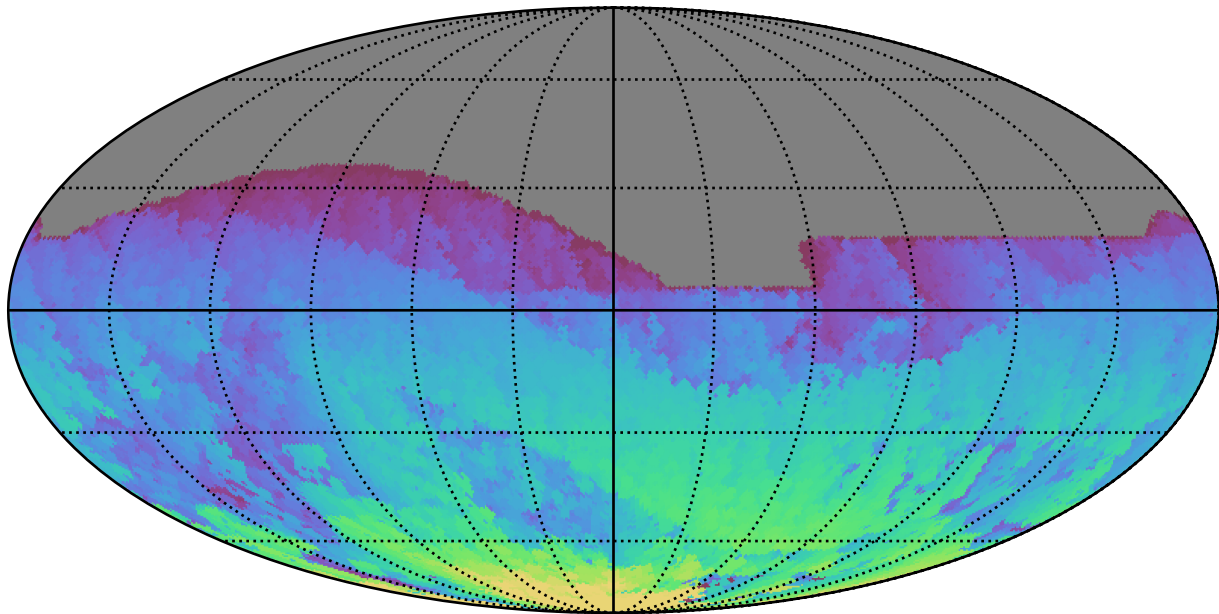
too_elab_r8_d2_giz_v3.4_10yrs All sky i band: Max HA
