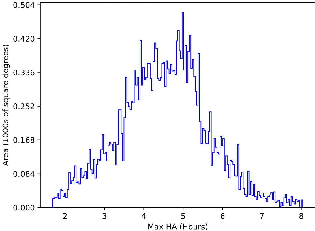
too_elab_r8_d2_giz_v3.4_10yrs All sky i band: Max HA
