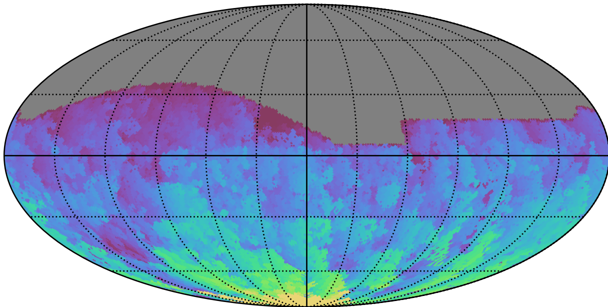
too_elab_r8_d2_giz_v3.4_10yrs All sky g band: Max HA
