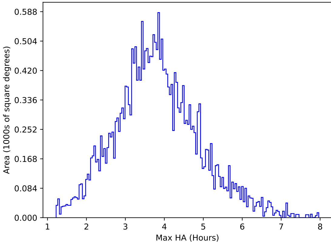
too_elab_r8_d2_giz_v3.4_10yrs All sky g band: Max HA
