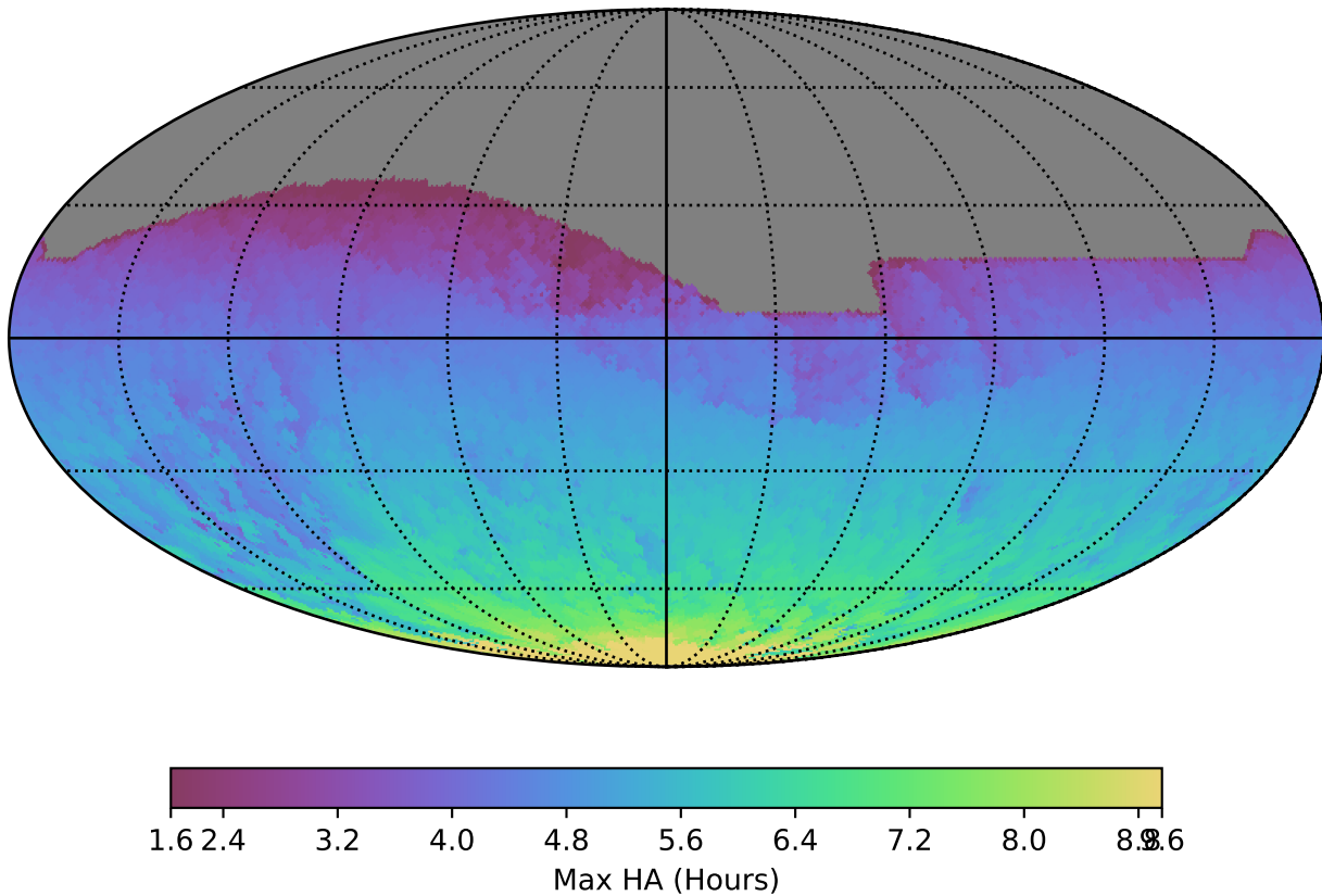
too_elab_r8_d2_giz_v3.4_10yrs All sky all bands: Max HA
