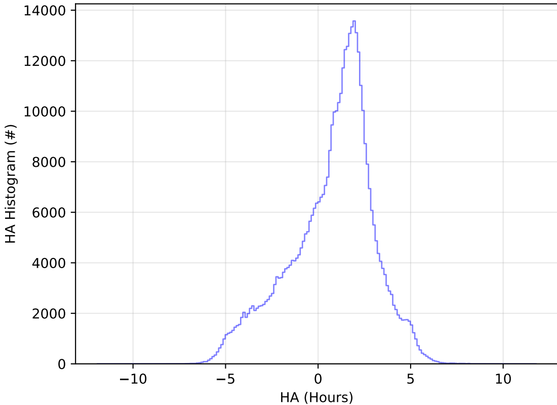
too_elab_r8_d2_giz_v3.4_10yrs WFD z band: HA Histogram
