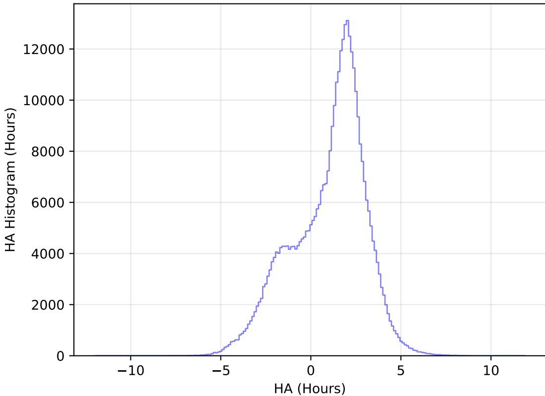
too_elab_r8_d2_giz_v3.4_10yrs WFD y band: HA Histogram
