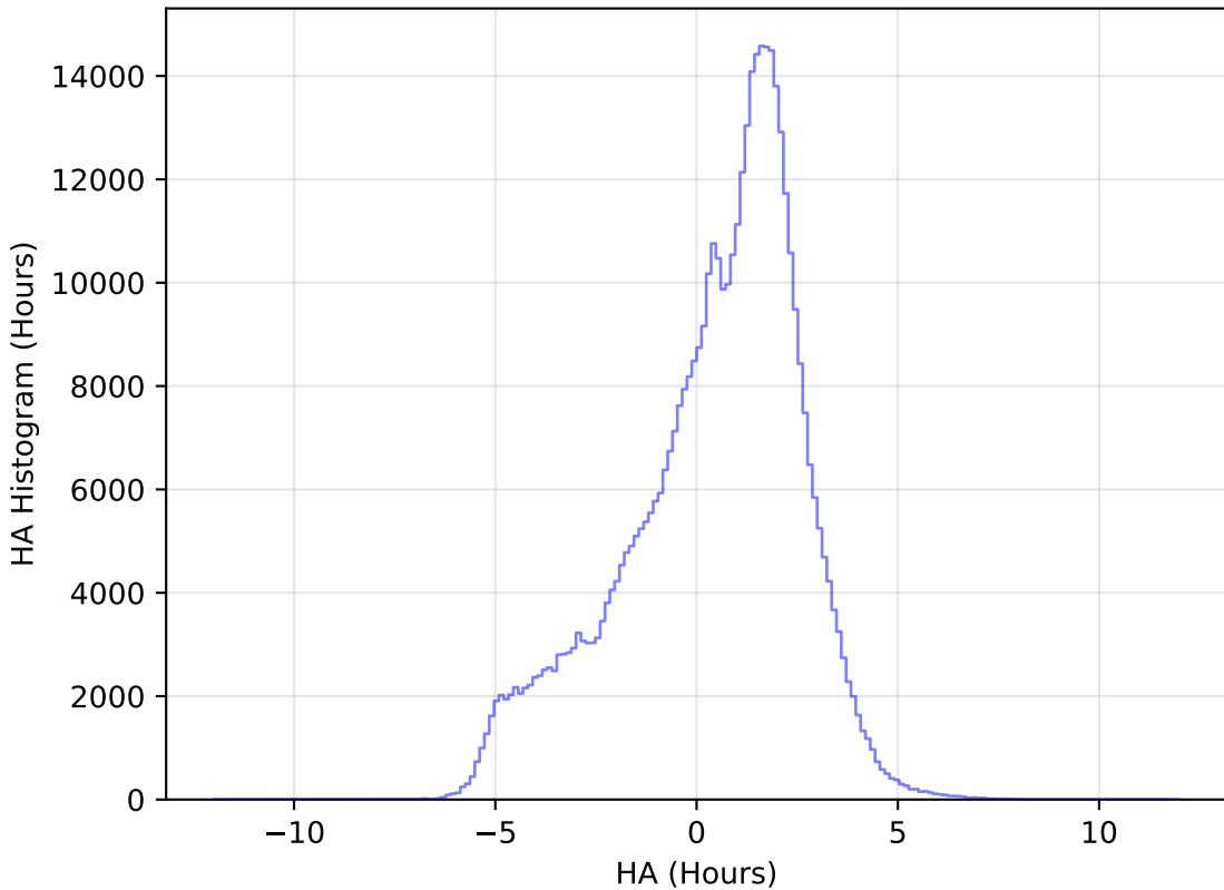
too_elab_r8_d2_giz_v3.4_10yrs WFD r band: HA Histogram
