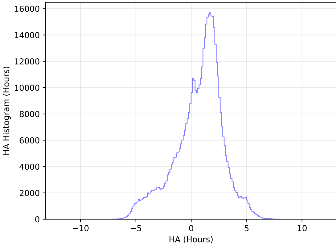
too_elab_r8_d2_giz_v3.4_10yrs WFD i band: HA Histogram
