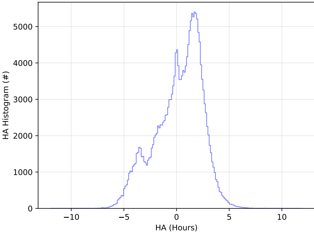
too_elab_r8_d2_giz_v3.4_10yrs WFD g band: HA Histogram
