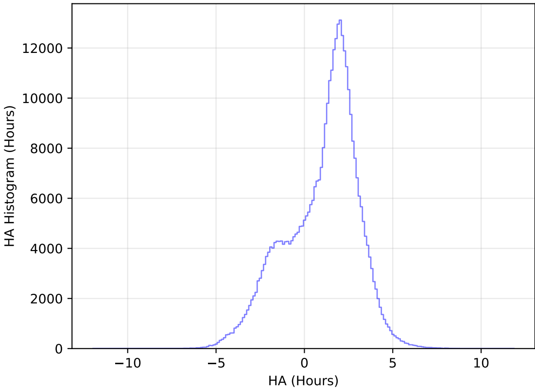
too_elab_r8_d2_giz_v3.4_10yrs All sky y band: HA Histogram
