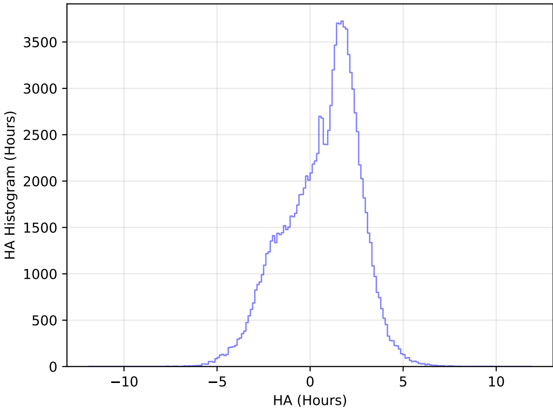
too_elab_r8_d2_giz_v3.4_10yrs All sky u band: HA Histogram
