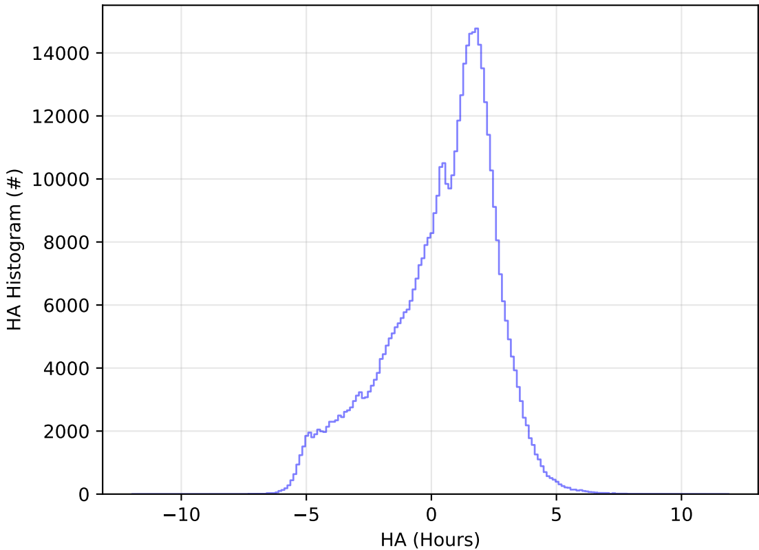
too_elab_r8_d2_giz_v3.4_10yrs All sky r band: HA Histogram
