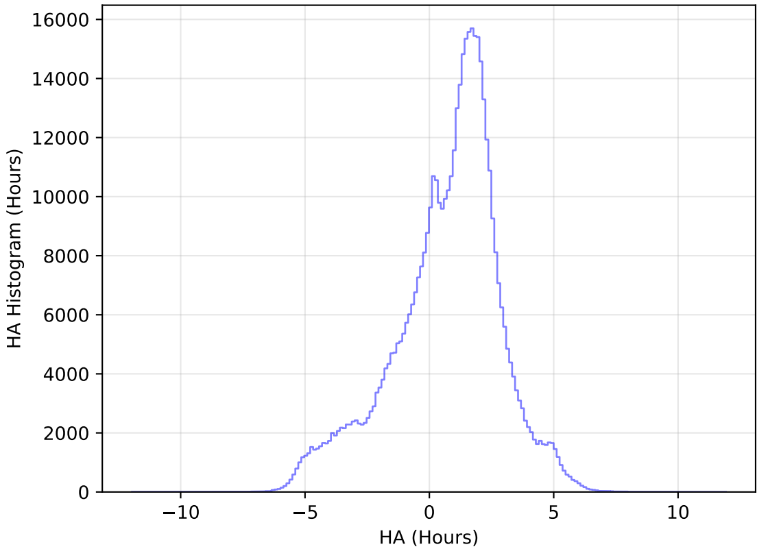
too_elab_r8_d2_giz_v3.4_10yrs All sky i band: HA Histogram
