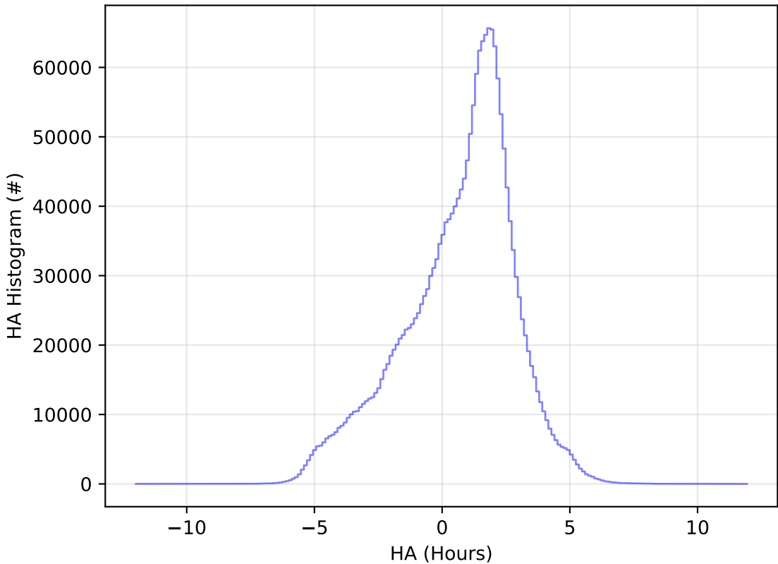
too_elab_r8_d2_giz_v3.4_10yrs All sky all bands: HA Histogram
