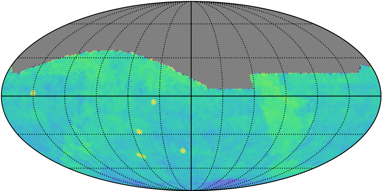
too_elab_r8_d2_giz_v3.4_10yrs gri All sky: Fraction of visits in pairs (10-60 min)
