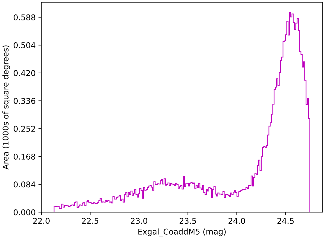
too_elab_r8_d2_giz_v3.4_10yrs Yr 1 z band: Exgal_CoaddM5
