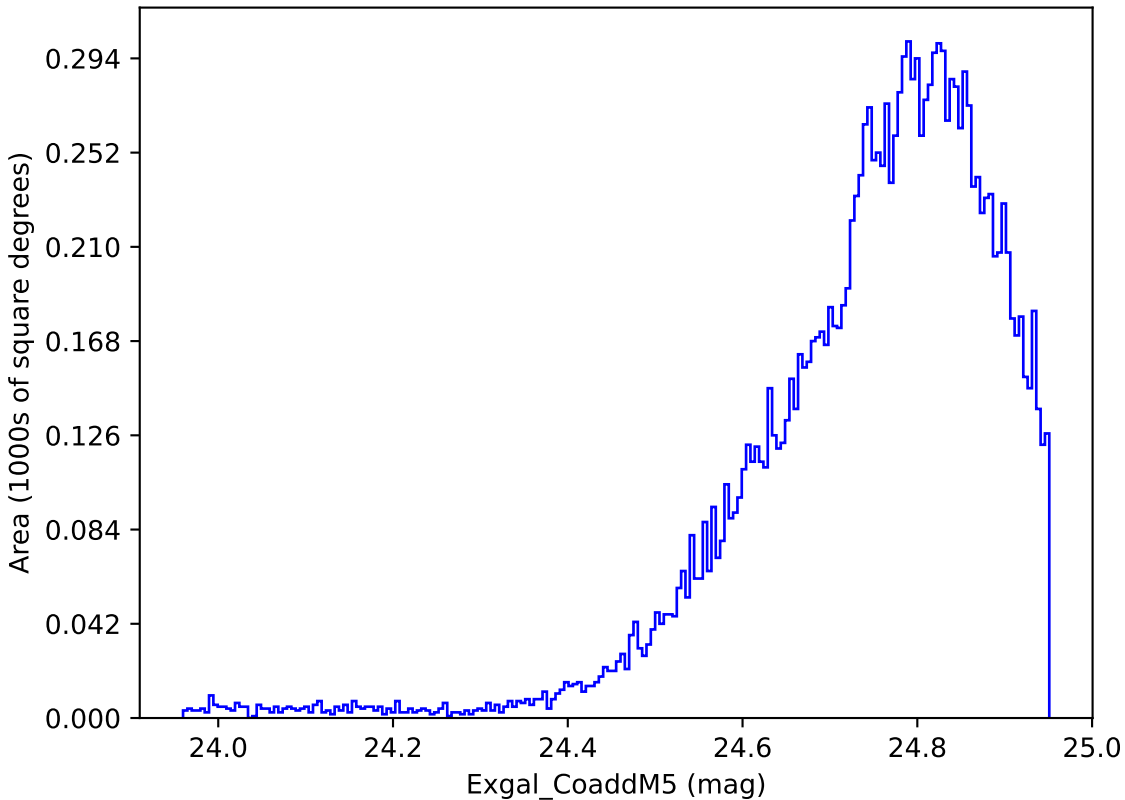
too_elab_r8_d2_giz_v3.4_10yrs WFD y band: Exgal_CoaddM5
