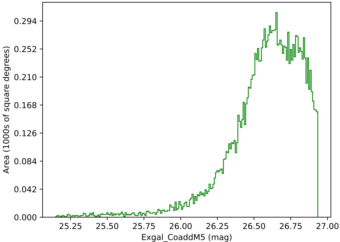
too_elab_r8_d2_giz_v3.4_10yrs WFD g band: Exgal_CoaddM5
