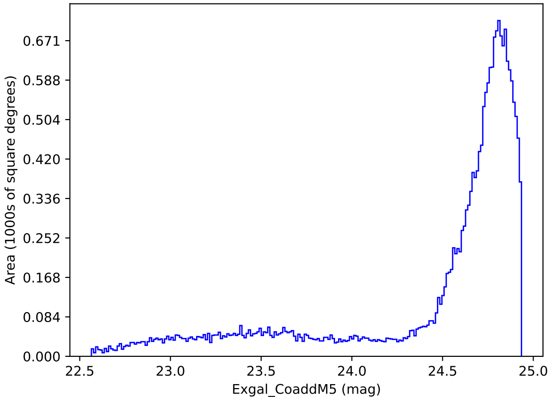
too_elab_r8_d2_giz_v3.4_10yrs All sky y band: Exgal_CoaddM5
