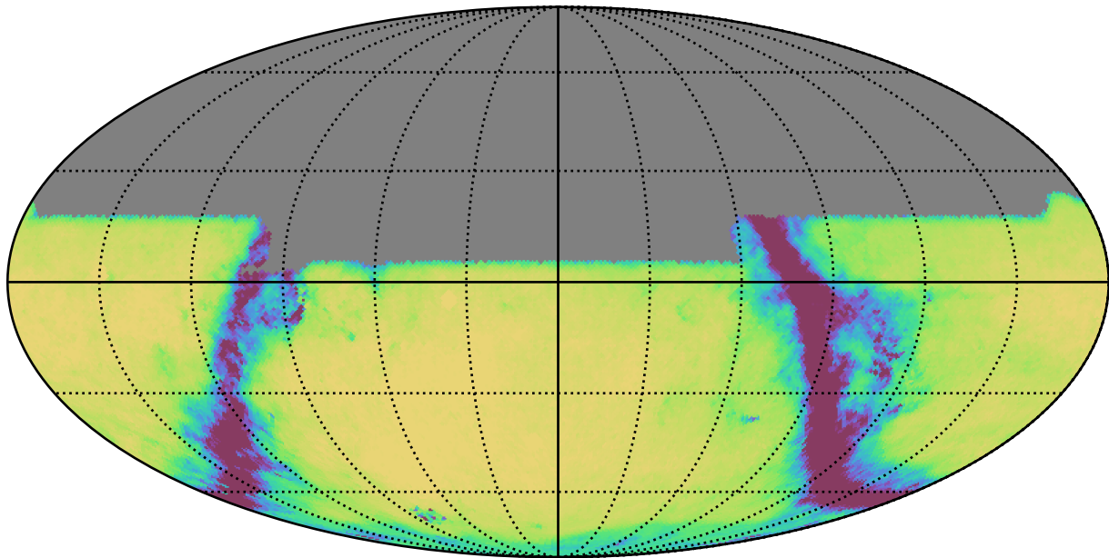
too_elab_r8_d2_giz_v3.4_10yrs All sky u band: Exgal_CoaddM5
