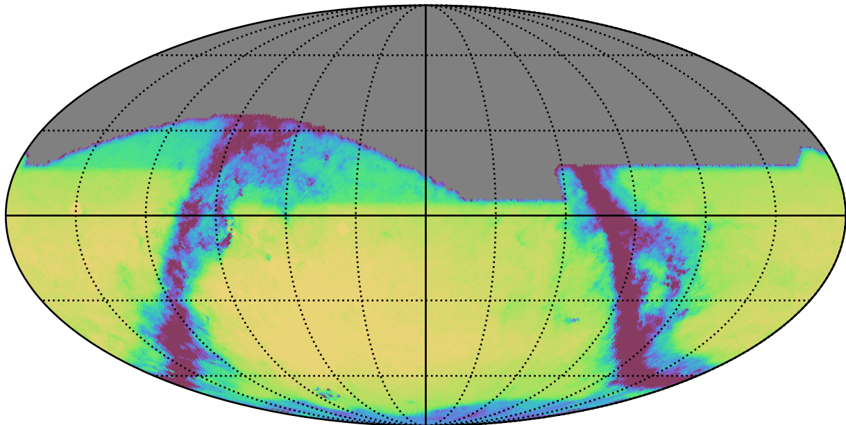
too_elab_r8_d2_giz_v3.4_10yrs All sky r band: Exgal_CoaddM5
