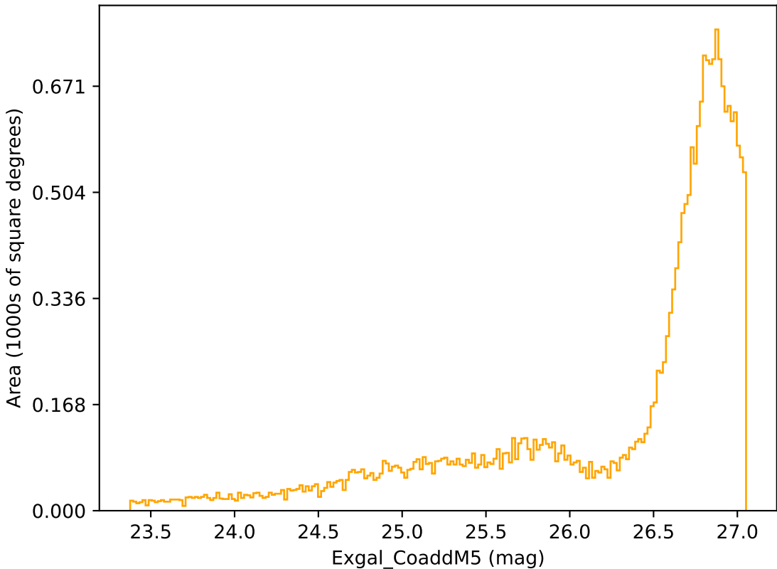
too_elab_r8_d2_giz_v3.4_10yrs All sky r band: Exgal_CoaddM5
