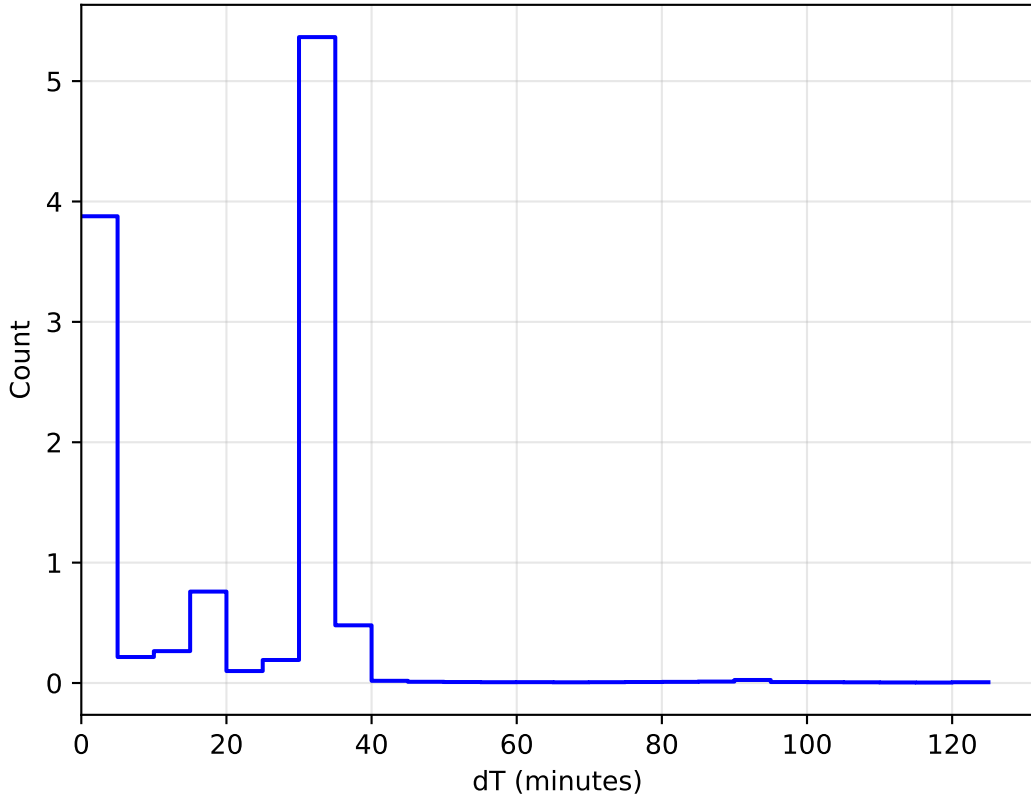
too_elab_r8_d2_giz_v3.4_10yrs WFD: DeltaT Histogram
