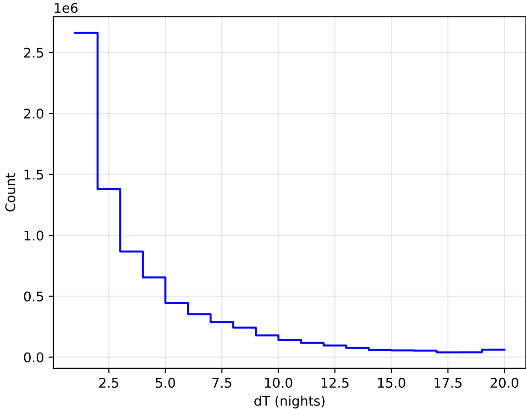
too_elab_r8_d2_giz_v3.4_10yrs WFD all bands: DeltaNight Histogram
