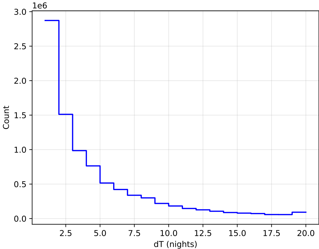
too_elab_r8_d2_giz_v3.4_10yrs All sky all bands: DeltaNight Histogram
