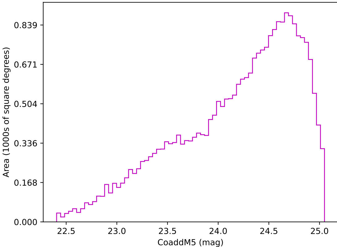
too_elab_r8_d2_giz_v3.4_10yrs Yr 3-4 z band: CoaddM5
